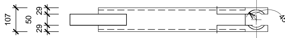
7 Extensions Back 1:10
