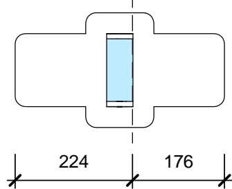
3 Ramp Base Plate Plan 1:10
